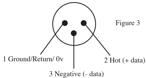
Male XLR Pin Configuration: US ITT Standard
